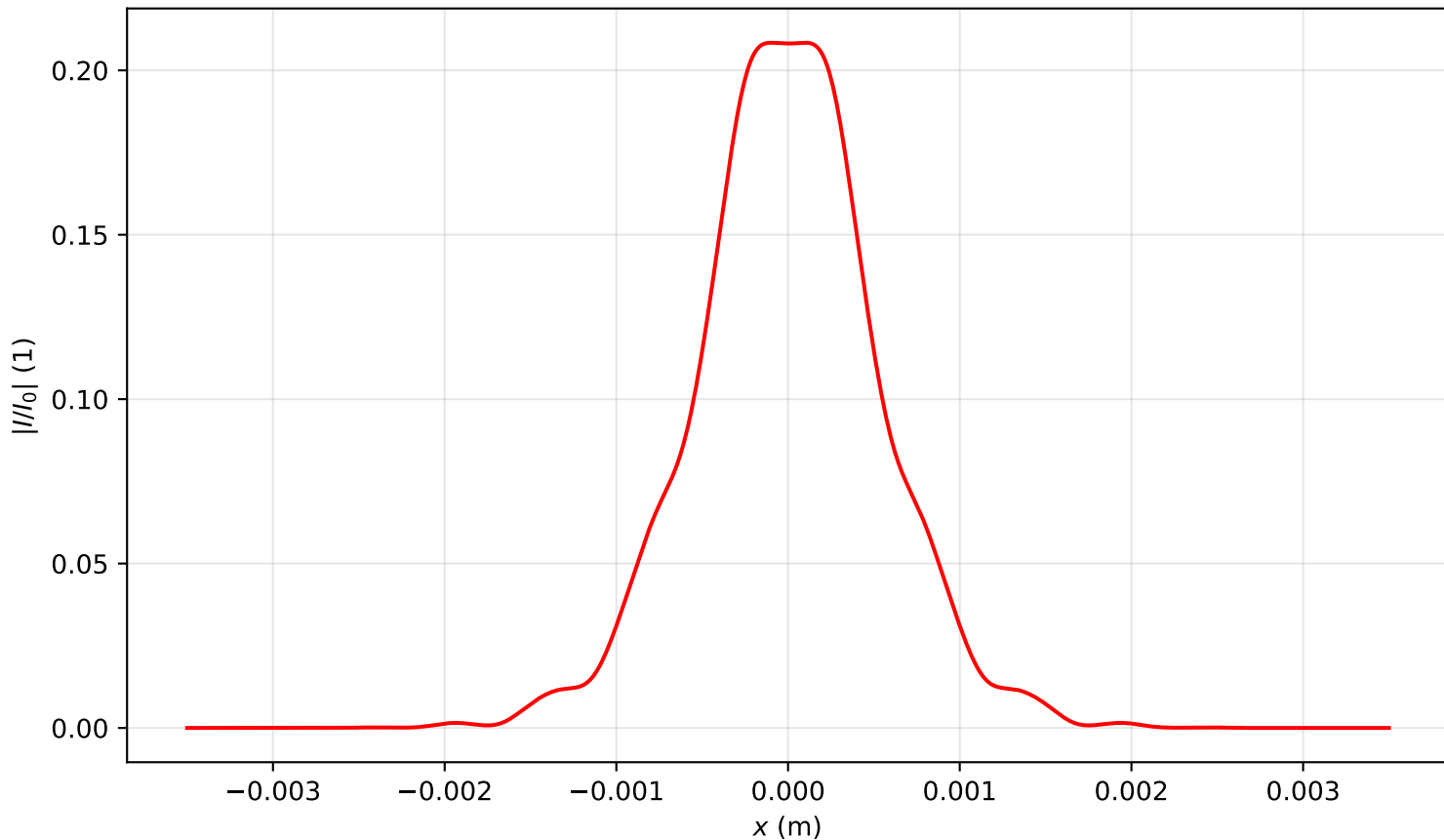
Intensity profile I(x, y = 0, z = 3.503)/I_0 , P_{in}=1.0P_{cr} , artificial time
